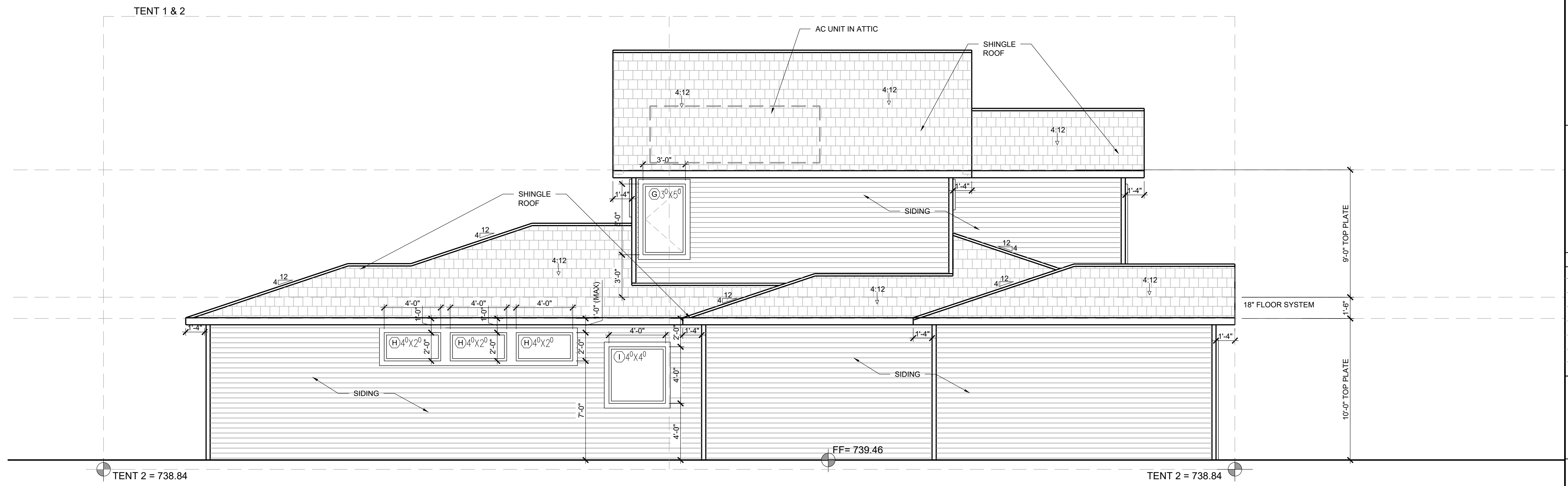
SIDE ELEVATION SCALE: 1/4" = 1'-0" (HALF SCALE = 1/8" = 1'-0")
